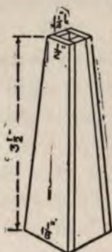
FIG. 296. Pedestal of Center-Table.
